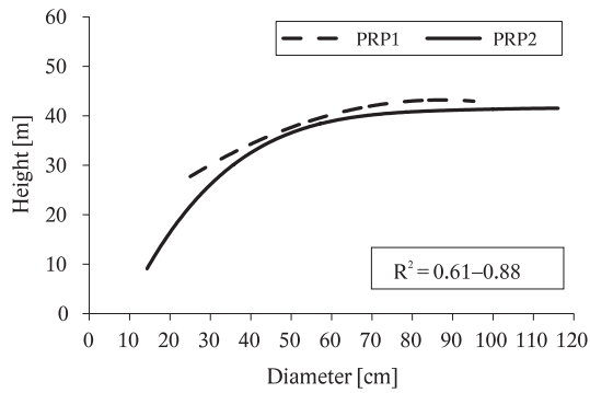
Fig. 3. The relationship between the breast height diameter and the height of beech on PRPs.
