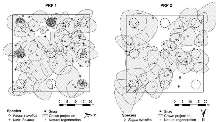
Fig. 5. Horizontal structure of the tree layer of the beech forest on PRPs in the Lány game enclosure.
