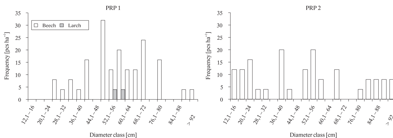
Fig. 2. Histograms of frequencies in diameter classes in the beech stands on the permanent research plots PRPs differentiated by tree species.
