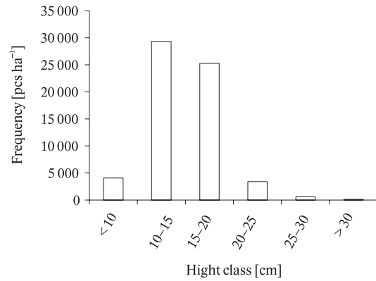
Fig. 4. Histogram of tree frequencies in height classes in the beech stand on PRP 1 in the Lány game enclosure.
