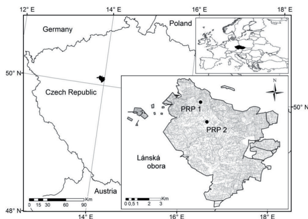
Fig. 1. The localisation of permanent research plots 1 and 2 in the Lány game enclosure.
