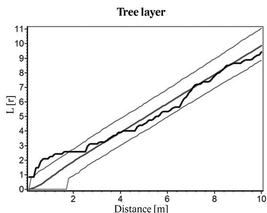
Fig. 6. Horizontal structure of the beech stand on PRP 1 in the Lány game enclosure expressed by L -function.
