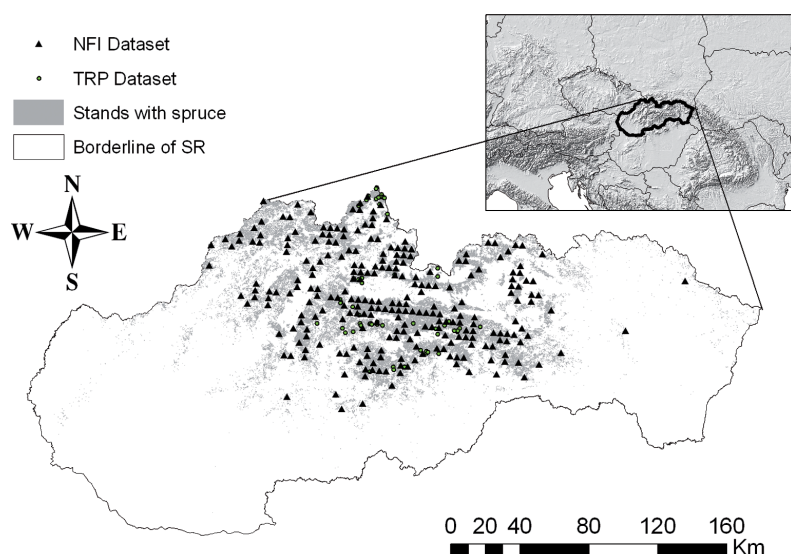
Fig. 1. Location and distribution of the plots from both the Slovakian NFI and TRP datasets.
