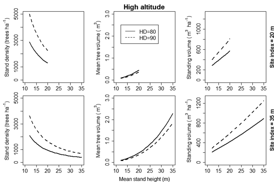
Fig. 5. Development of stand density, mean tree volume and standing volume per hectare at different HD ratios and different site indexes of spruce – at an altitude of 1200 m a.s.l.
