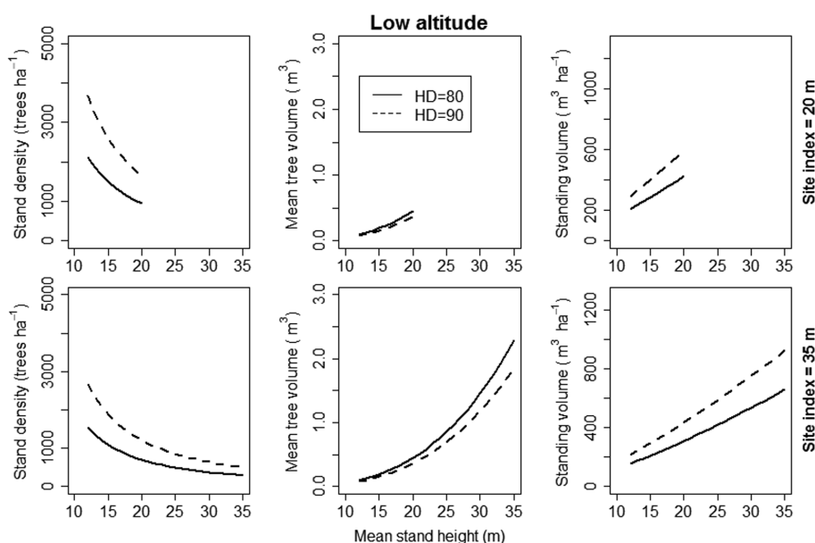
Fig. 4. Development of stand density, mean tree volume and stand volume per hectare at different HD ratios and different site indexes of spruce – at an altitude of 800 m a.s.l.
