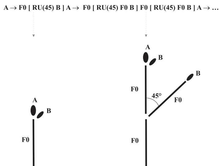
Fig. 2. Development of geometrical structures specified by the growth grammar A \Rightarrow F0 [ RU(45) B ] A ; B \Rightarrow F0 B . Horizontal arrows stand for rule application, dotted vertical arrows for interpretation of the strings by the turtle
